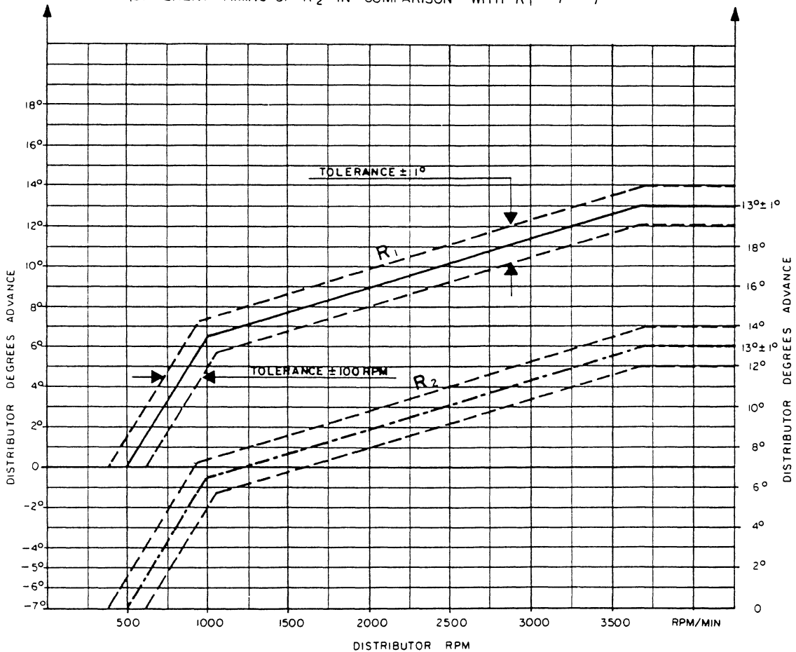
AUTOMATIC ADVANCED CURVE OF THE DISTRIBUTOR (DIFFERENT TIMING OF R 2 IN COMPARISON WITH R 1 - 7° -)
