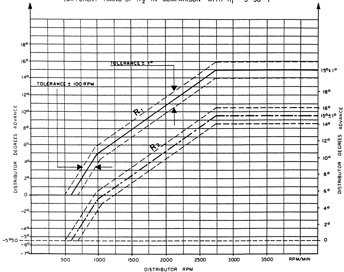
AUTOMATIC ADVANCED CURVE OF THE DISTRIBUTOR (DIFFERENT TIMING OF R_2 IN COMPARISON WITH R_1 - 5^\circ 30' )
